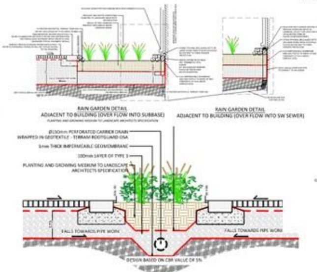
TYPICAL RAIN GARDEN DETAIL WITHIN PAVING PLANTING AND GROWING MEDIUM TO LANDSCAPE ARCHITECTS SPECIFICATION
