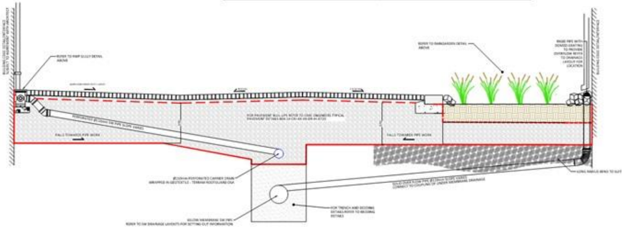
TYPICAL SECTION THROUGH STREET PLANTING AND GROWING MEDIUM TO LANDSCAPE ARCHITECTS SPECIFICATION SCALE: 1/5
