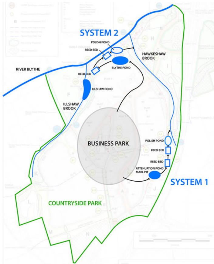
Figure 2: Blythe Valley Park SuDS
