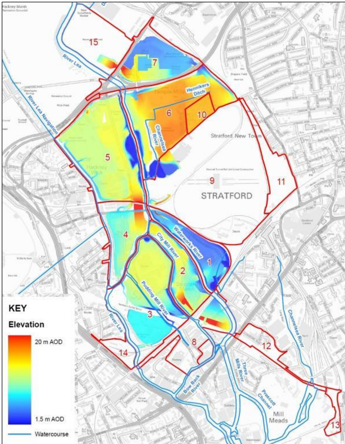
Figure 3 Olympic & legacy topography scheme (Barry Plowright)
