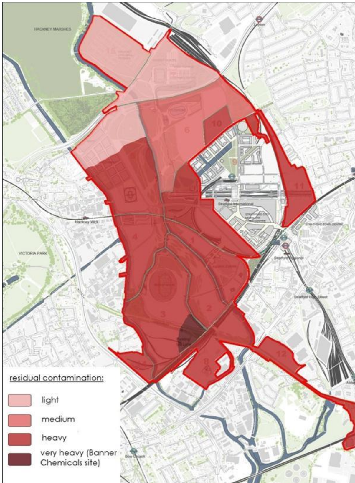
Figure 1 Anticipated residual level of contamination post remediation works (Barry Plowright)
