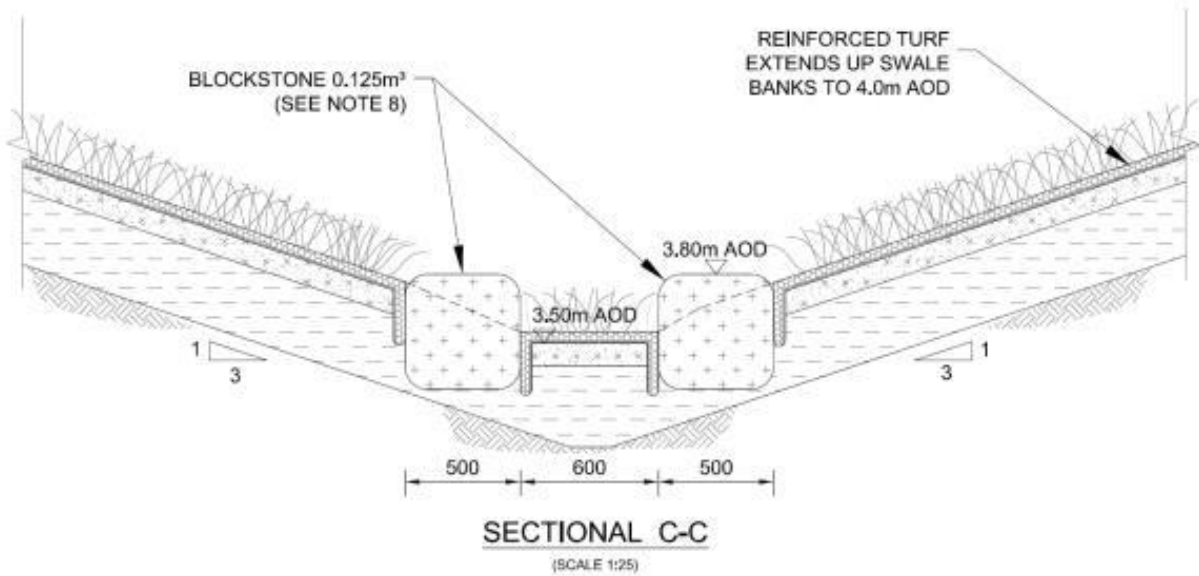
Figure 8 Cross Section through swale & check dam (Barry Plowright)
