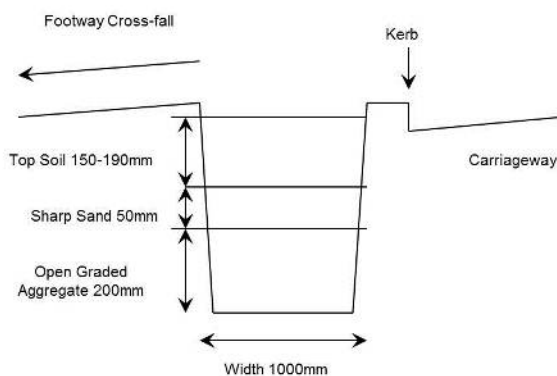
Figure 4 Grass verge construction detail Central Hill
